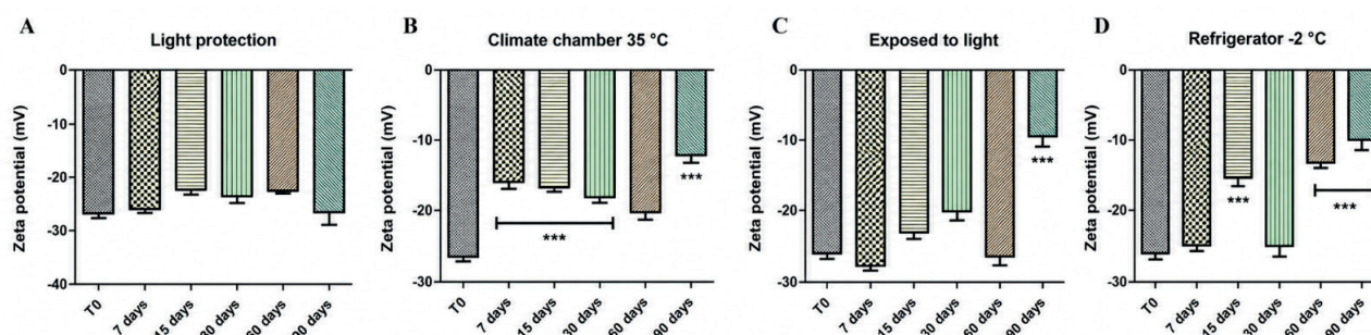
Figure 4 - Results of the stability analysis regarding the zeta potential of nanoparticles over 90 days and under different storage conditions: amber glass container protected from light (Fig. 4-A), amber glass container in a climatic chamber at \pm 35 °C (Fig. 4-B), transparent glass container exposed to light (Fig. 4-C), and amber glass container under refrigeration at - 2 °C (Fig. 4-D).
